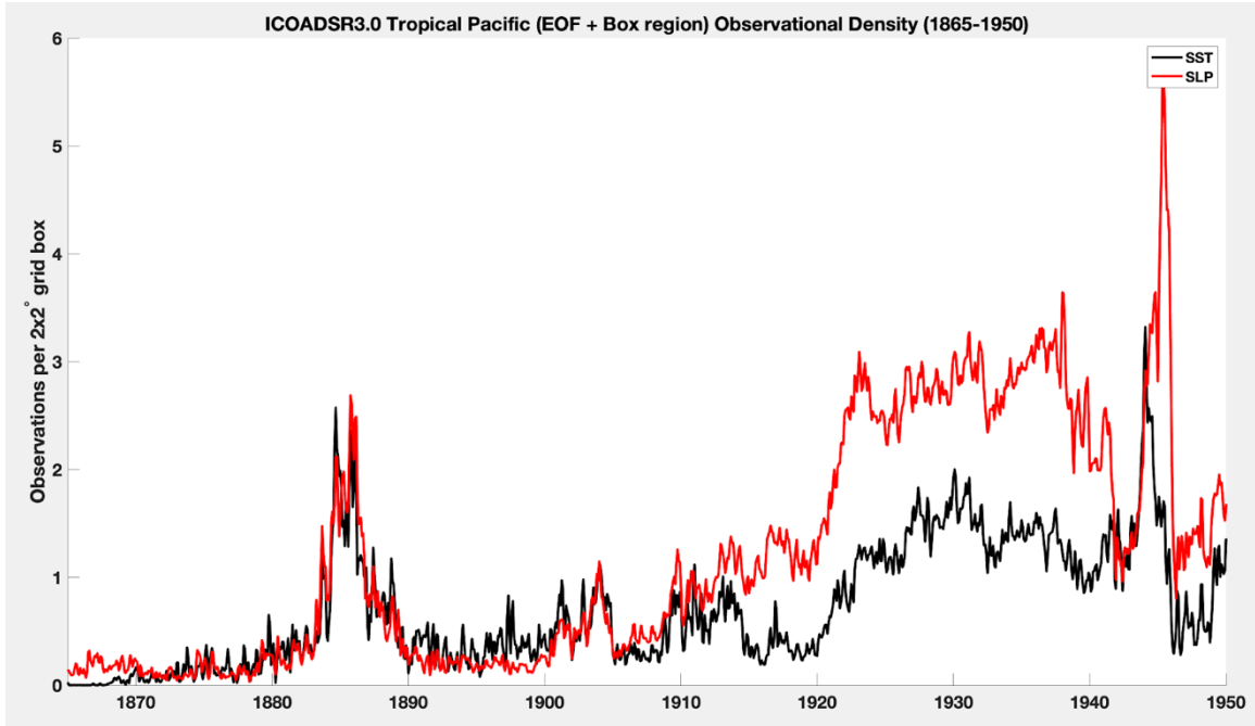
Figure 13. ICOADSR3.0 Tropical Pacific SST (black) and SLP (red) Number of Bi-Monthly Observations per 2 \times 2^\circ grid box averaged over their EOF (SST: [15S-10N, 160E-80W], SLP: [30S-20N, 100E-80W]) and Box (SST: [5S-5N, 180W-80W], SLP: Tahiti [17.7S, 149.4W], Darwin [12.5S, 130.8E] (1865-1950).
