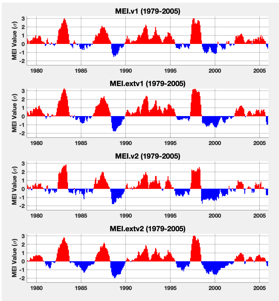
Figure 25. MEI anomaly time series (1979-2005): MEI.v1 (top), MEI.ext (second from top), MEI.v2 (second from bottom), and MEI.extv2 (bottom)
