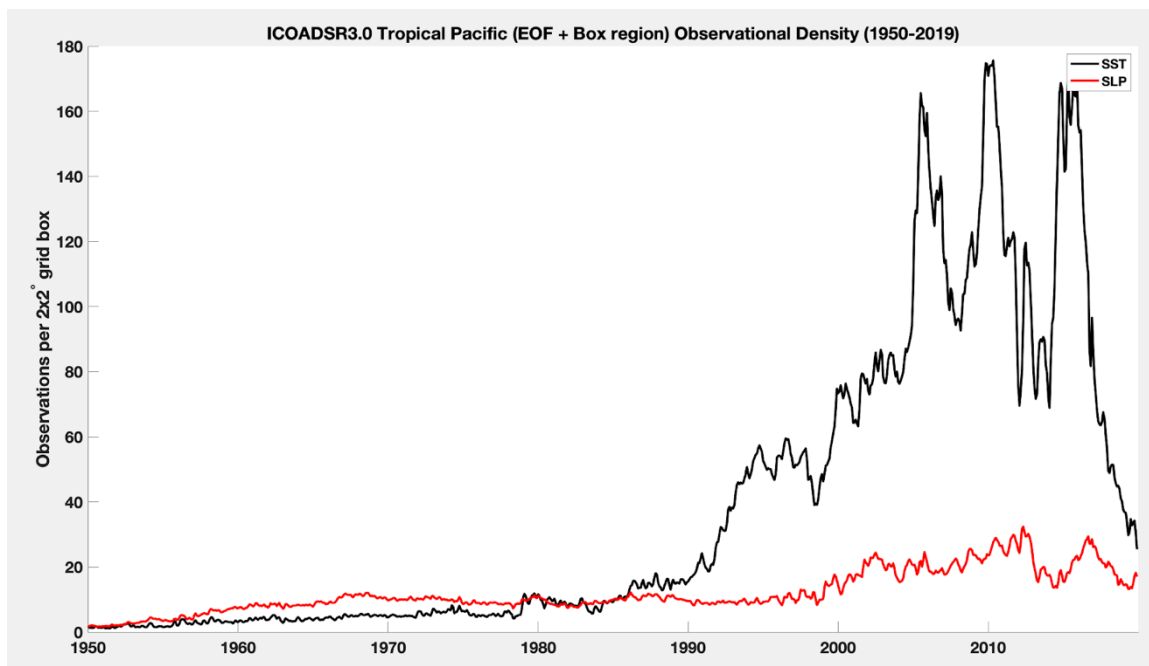
Figure 14. ICOADSR3.0 Tropical Pacific SST (black) and SLP (red) Number of Bi-Monthly Observations per 2 \times 2^\circ grid box averaged over their EOF (SST: [15S-10N, 160E-80W], SLP: [30S-20N, 100E-80W]) and Box (SST: [5S-5N, 180W-80W], SLP: Tahiti [17.7S, 149.4W], Darwin [12.5S, 130.8E] (1950-2019).
