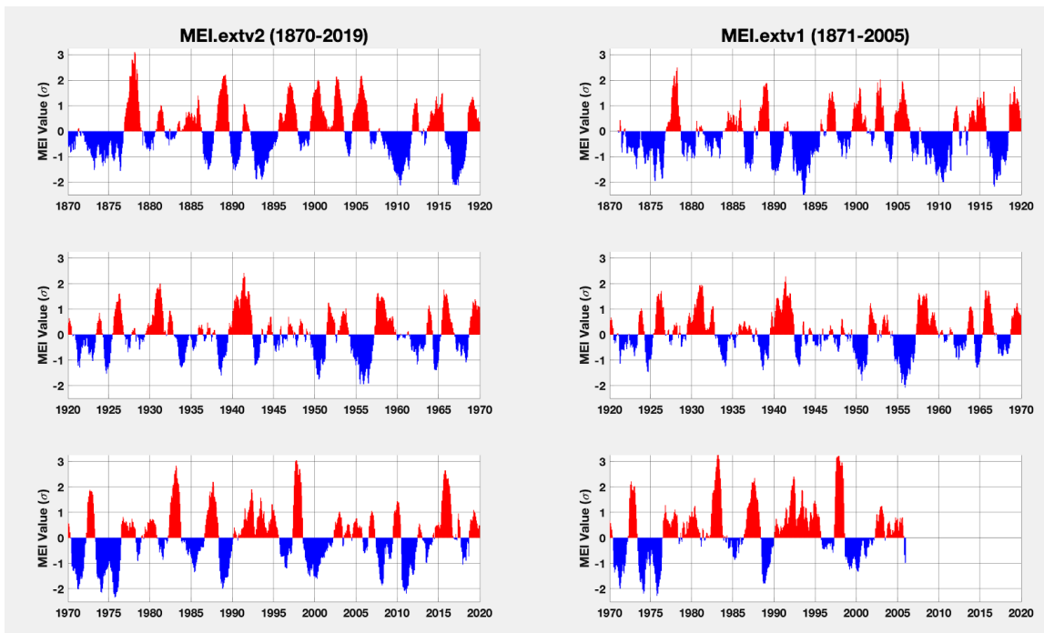
Figure 23. Time series of the MEI.extv2 (left) and MEI.extv1 (right). Red/warm (Blue/cool) colors are associated with El Nino (La Nina) conditions. The overall structure of the plot was motivated by and follows similar conventions to Wolter and Timlin (2011).
