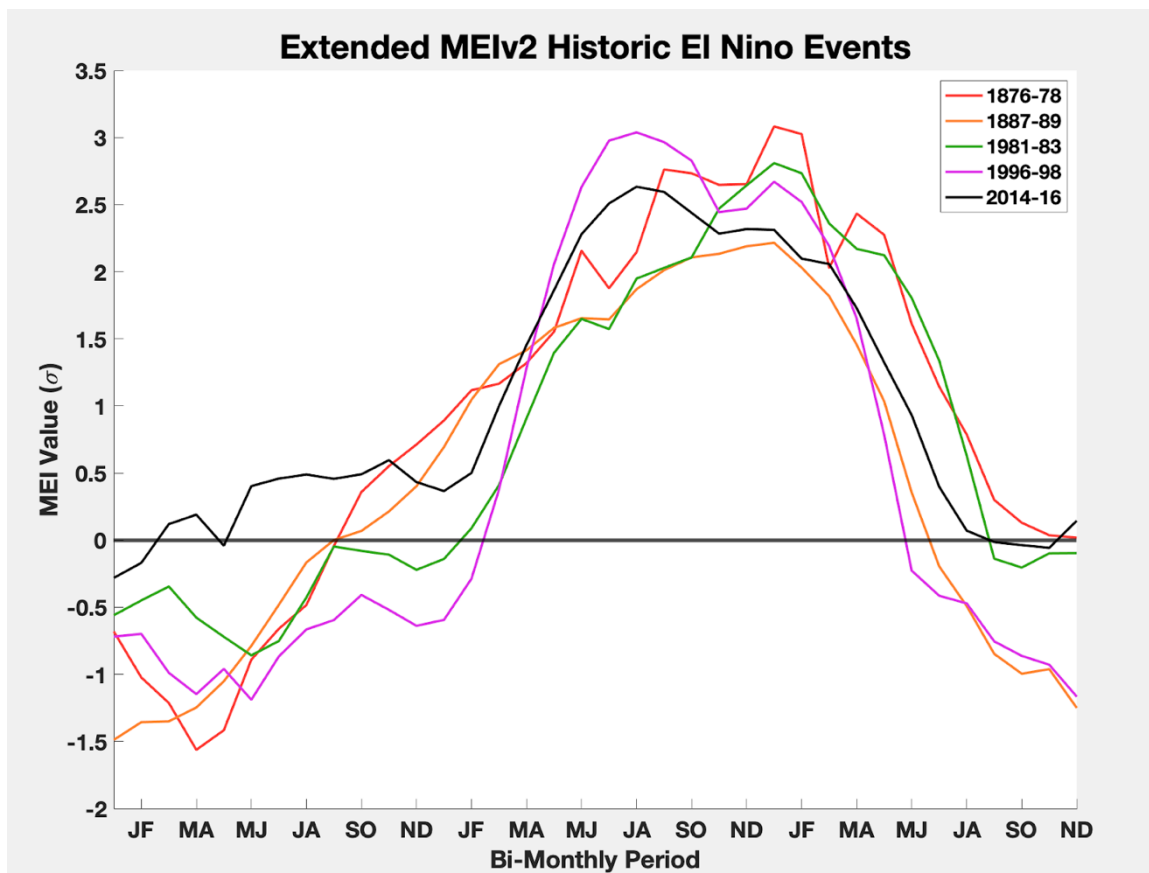
Figure 30. MEI.extv2 “historic” (top 5) El Nino events (as measured by the ensemble median)
