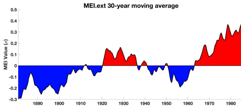
Figure 28. MEI.ext 30-year moving average values (red = positive/El Nino bias, blue = negative/La Nina bias).
