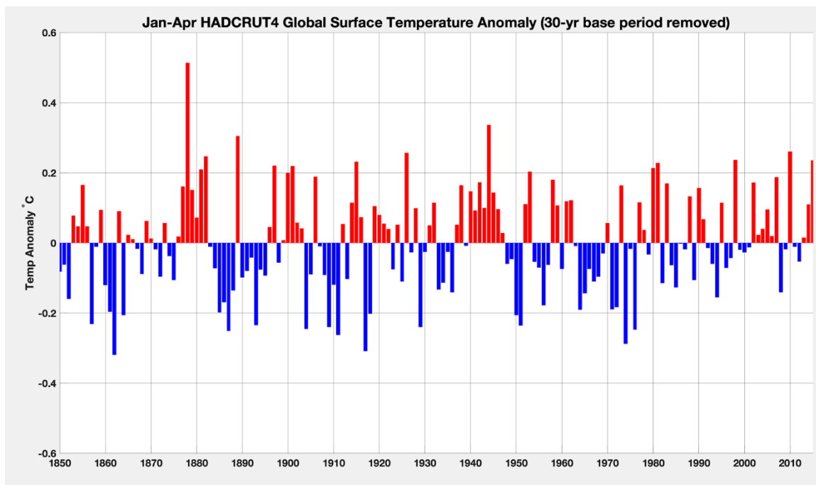
Figure 22. Jan-April averaged HADCRUT4 global surface temperature anomaly average, with a 30-year sliding base period removed (motivated by Aceituno et al, 2009).
