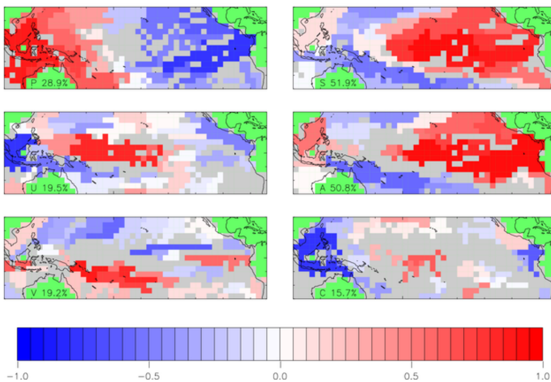
Figure 5. Oct-Nov MEI.v1 EOF-1 loadings for SLP (P) (top left), zonal wind (U) (middle left), meridional wind (V) (bottom left), SST (S) (top right), SAT (A) (middle right), Cloud fraction of sky (C) (bottom right). Taken from NOAA ESRL's MEI.v1 web page.
